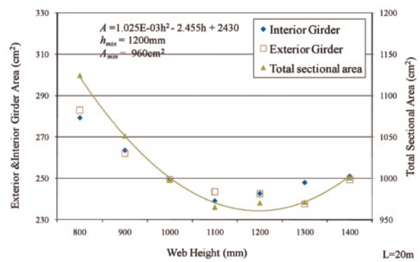
Figure 4 Optimum Girder Height for L=20m (with vertical stiffener, SM490)
