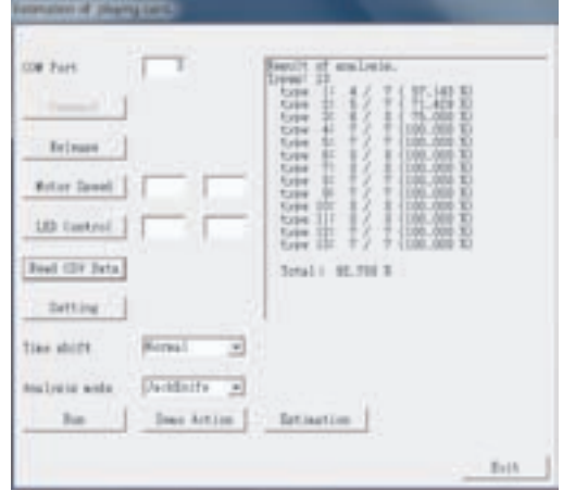
Figure 3. Example of Analyzed Result on COMPUTER by Canonical Discriminant Analysis.
