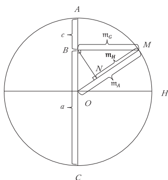
Fig. 1. A Circle and Three Types of Means
