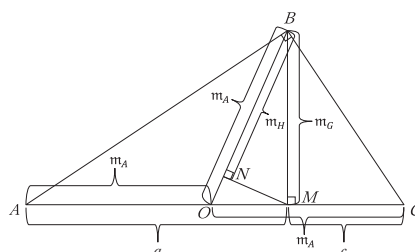
Fig. 2. A Right Triangle and Three Types of Means
